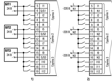
1) ПР110–24.12Д.8P 2) ПР110–220.12ДФ.8P
