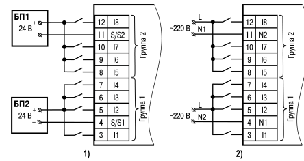
1) ПР110–24.8Д.4P 2) ПР110–220.8ДФ.4P
